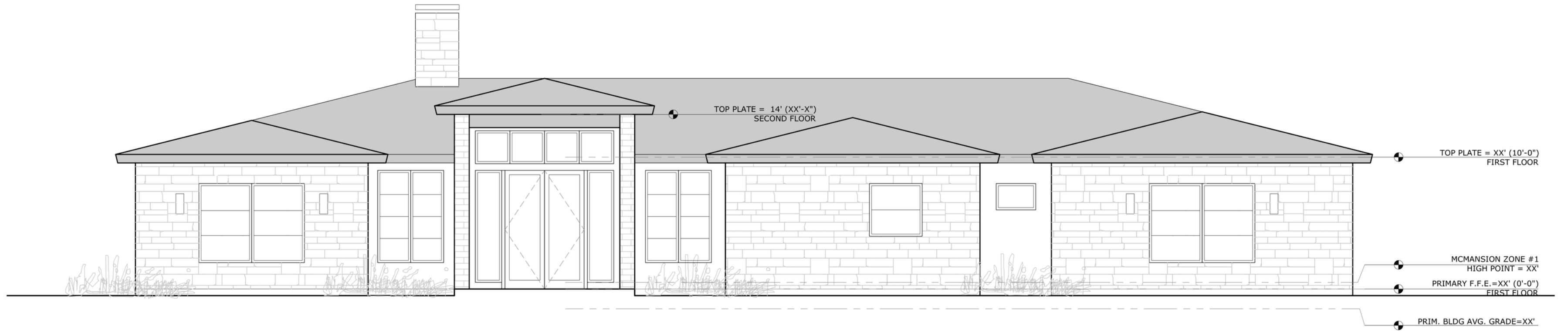
02 North Elevation - Front 1/4" = 1'-0" @ 22x34 1/8" = 1'-0" @ 11x17
